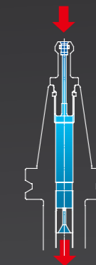
BT 中心出水 Center-Through Coolant Type for BT Shank
